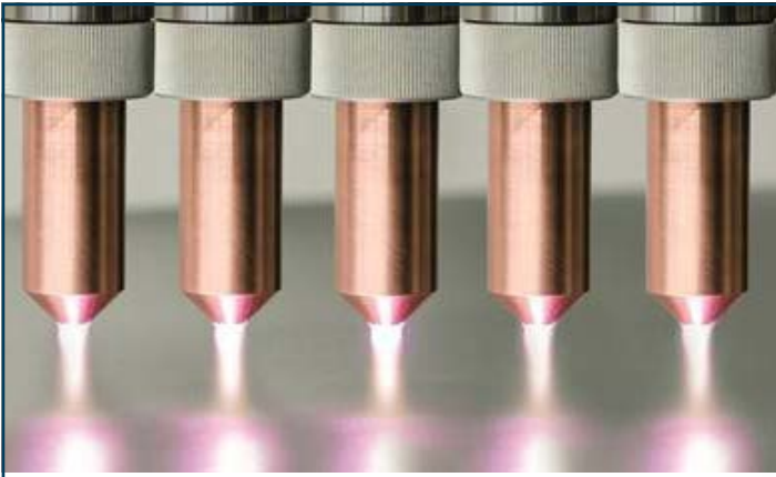
Multi-channel process: 5 plasma generators (type PN3) in compressed-air operation
